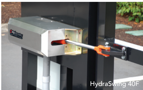
HydraSwing 40/Twin 4,000 lb gate up to 24 ft wide up to 16 ft wide Twin 15-20 second open
